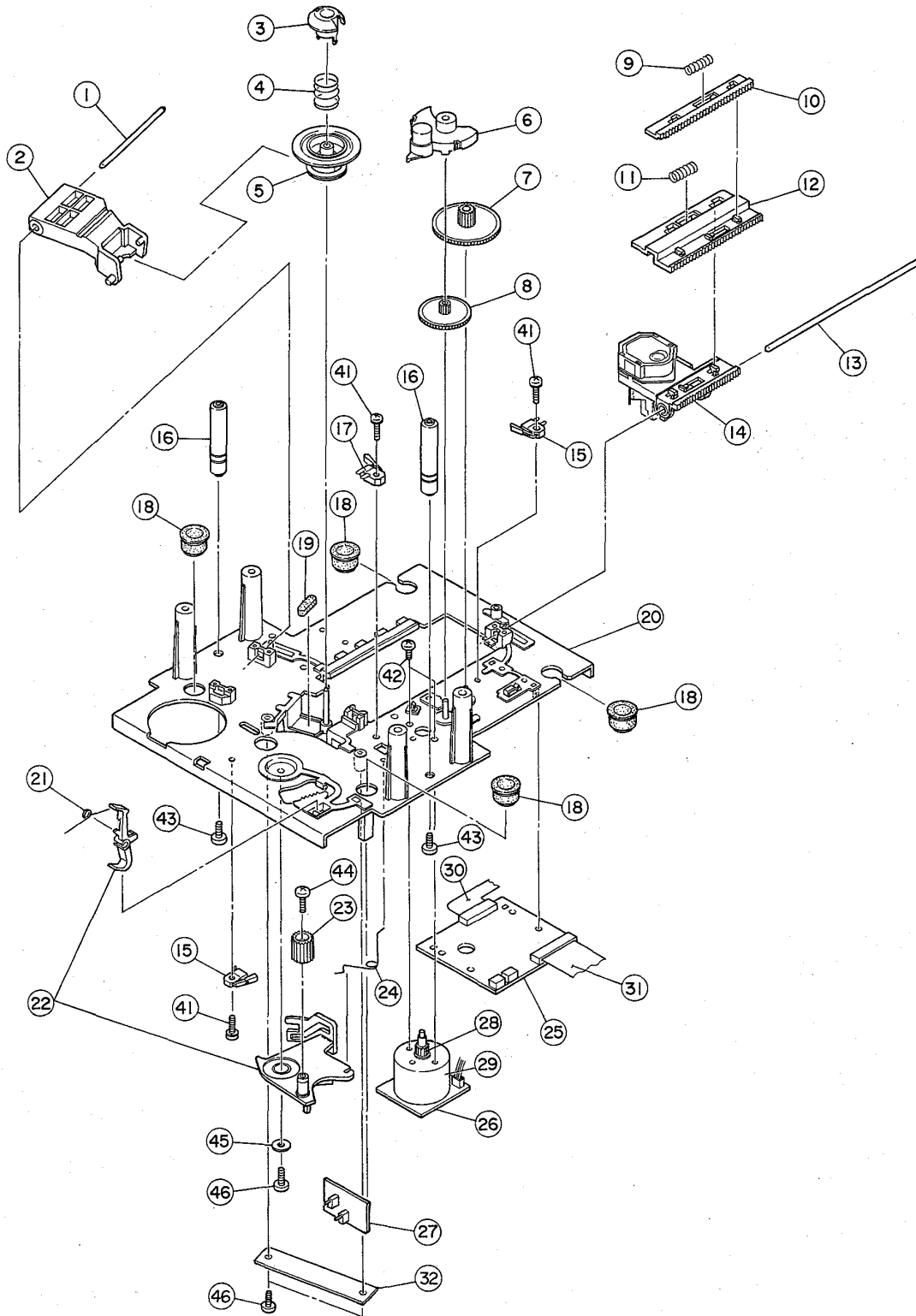
EXPLODED VIEW-3
