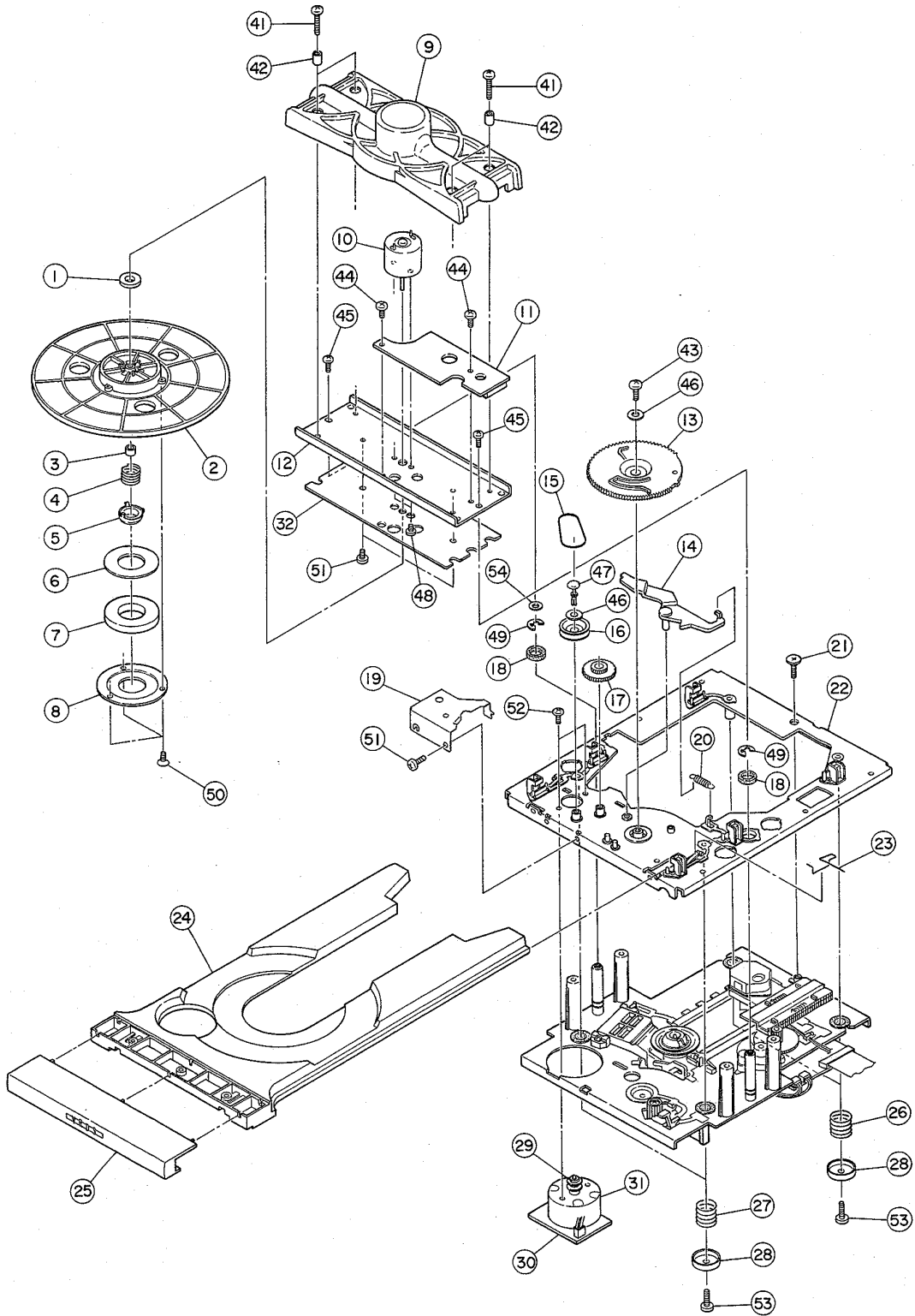
EXPLODED VIEW-2
